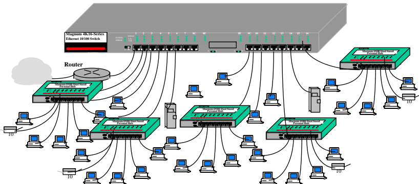
Fig. 2.4b: Magnum 4K16 Switch provides high bandwidth solution for small office or class room, offering expansion via “future-proof” fiber.
